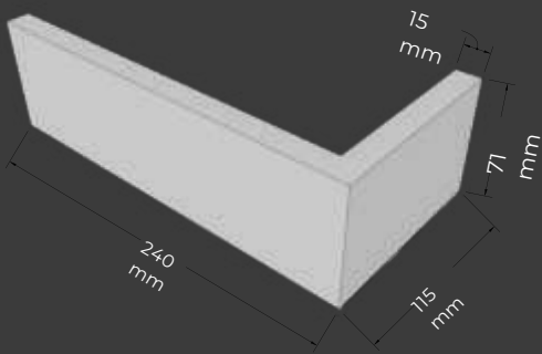
Winkelriemchen Thin Brick Corner
